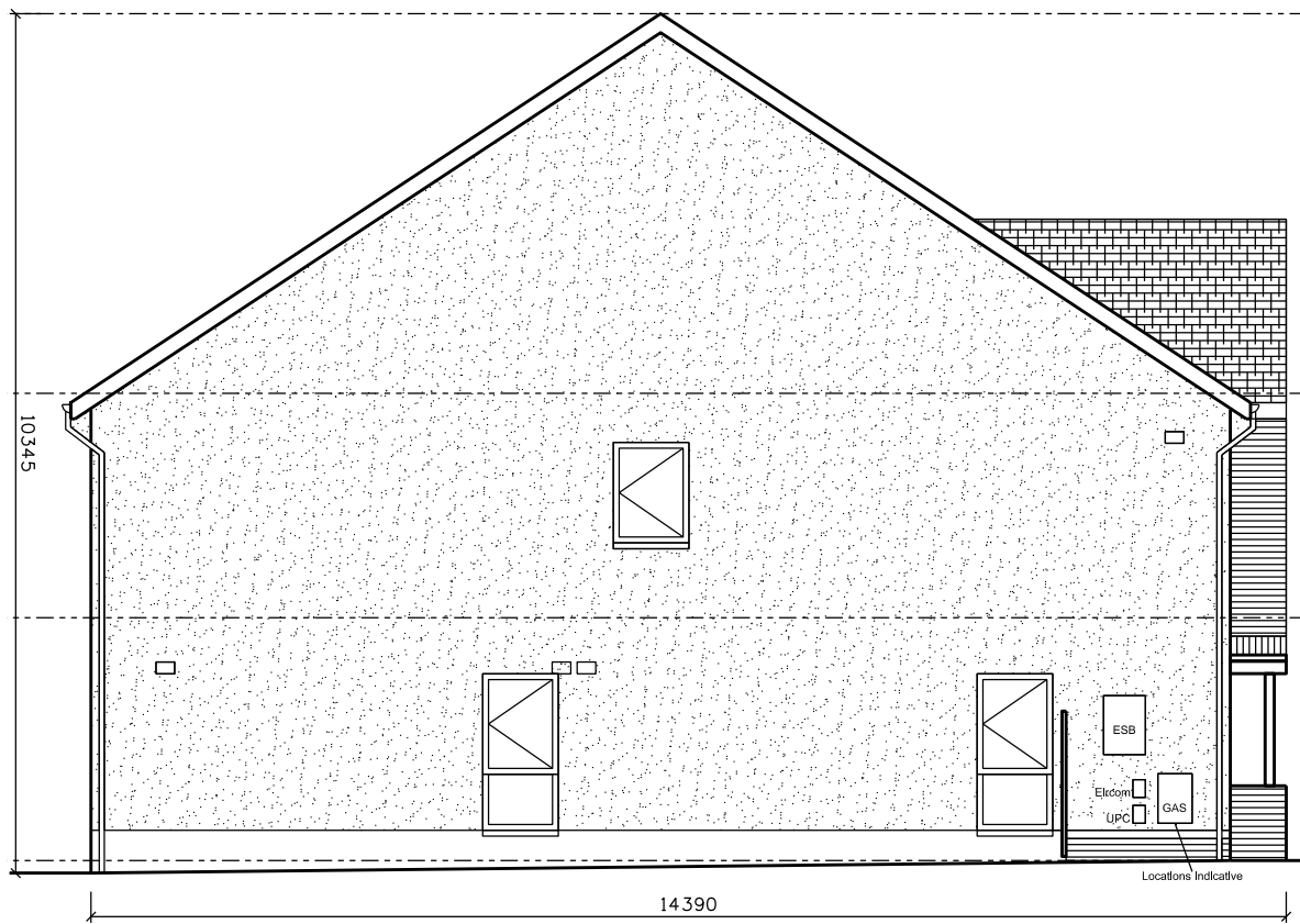
SIDE ELEVATION
