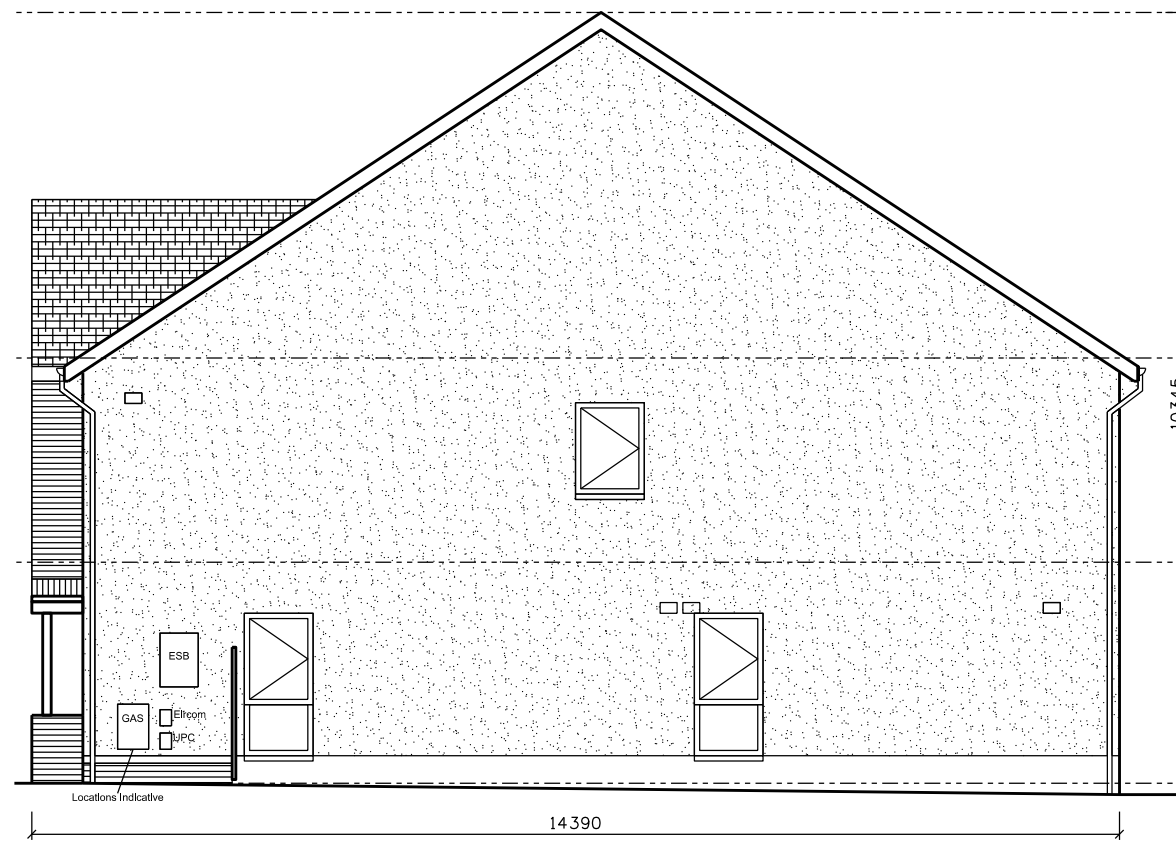
SIDE ELEVATION
